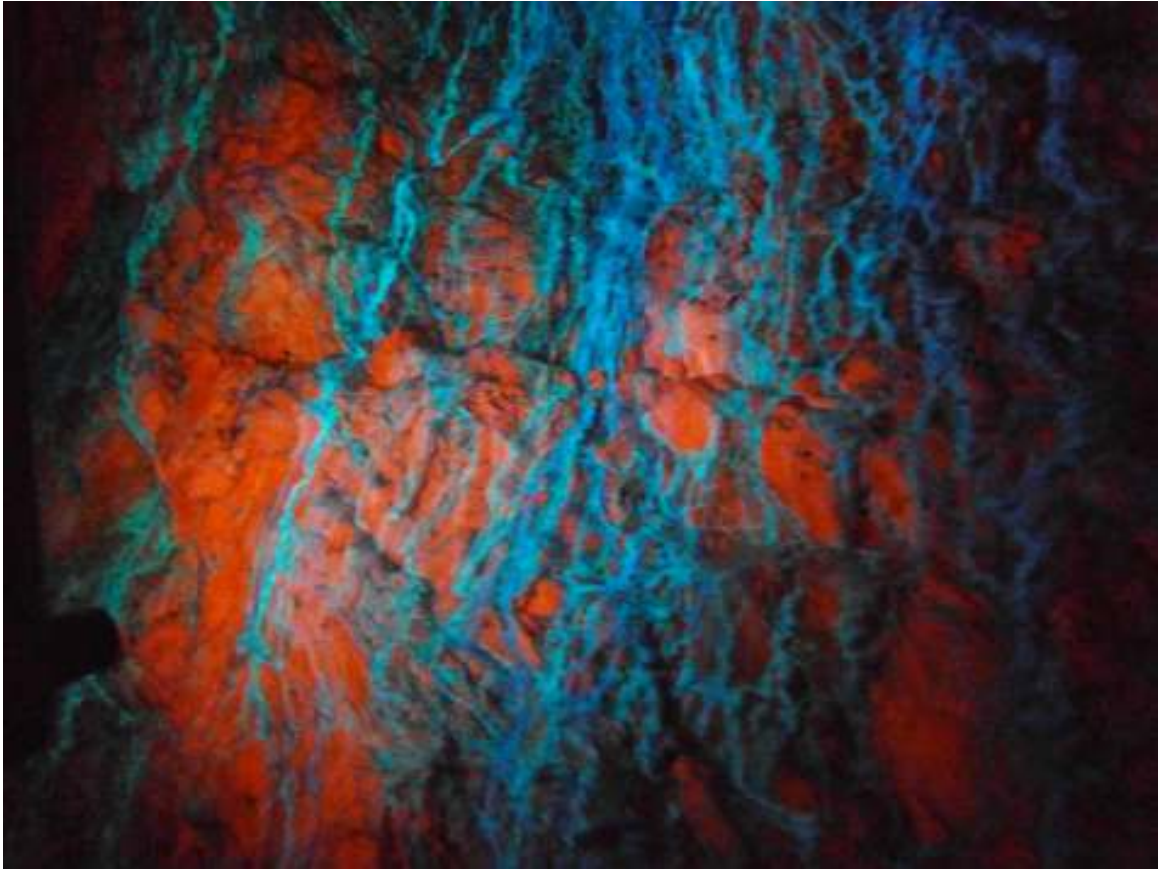
Flowstone over fluorescent calcite
