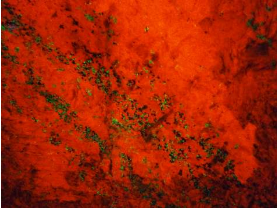
Calcite and Willemite veins
