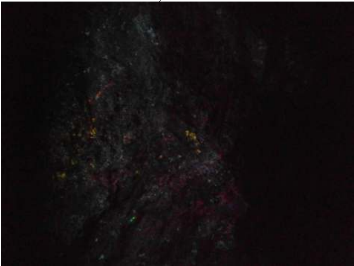
The wall of Sphalerite
