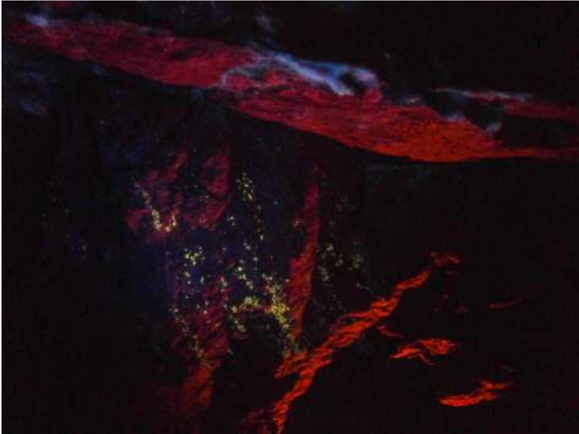
Veins and faults in the calcite wall
